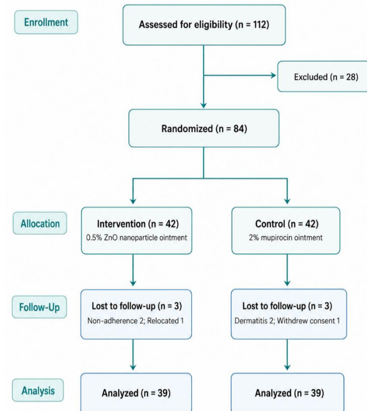
Figure 1 CONSORT Flowchart
